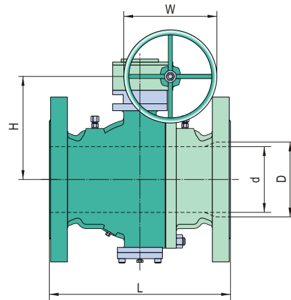
Reduced Bore Class 150
