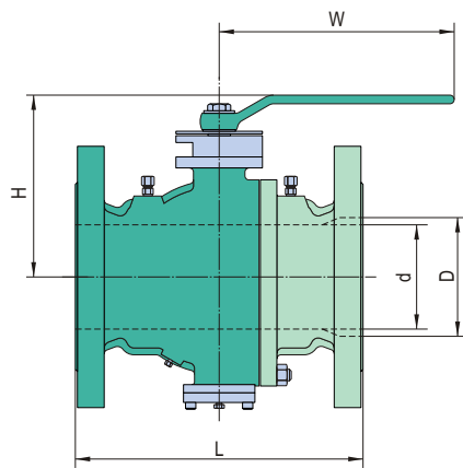
Full Bore Class 150
